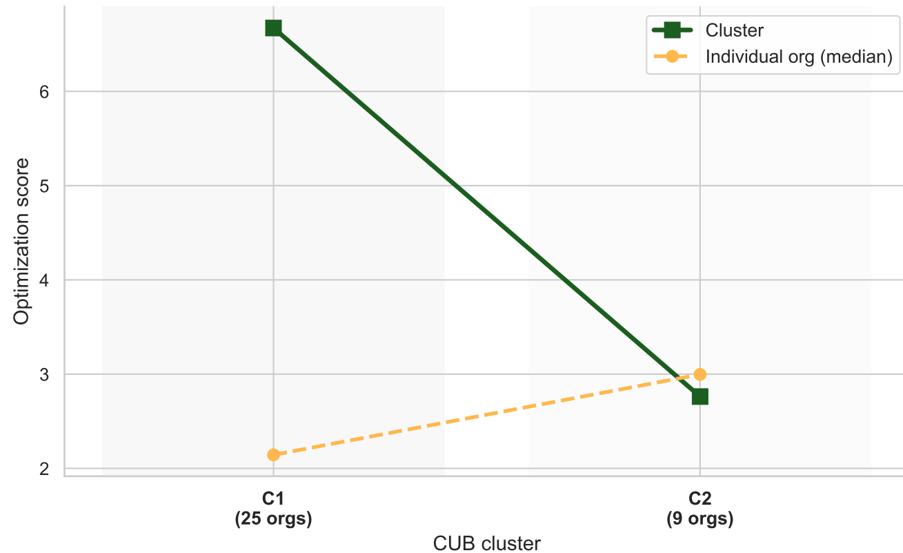
DBI-optimal k=2
