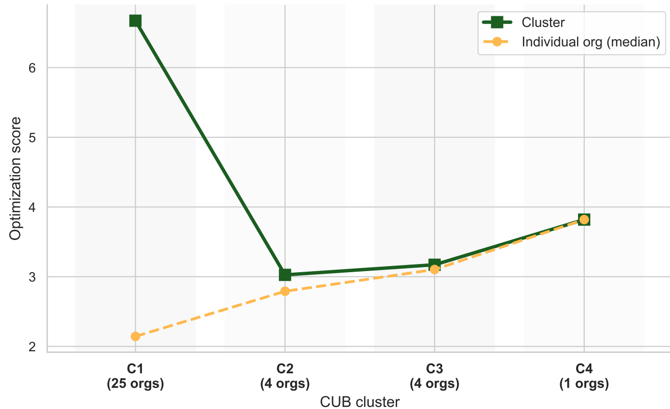
k=4 (forced)
