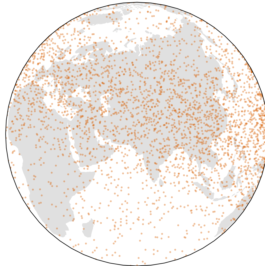
Varadhan
