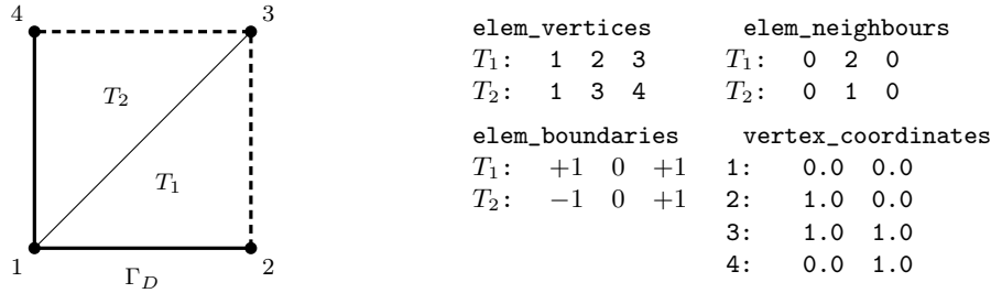
Figure 23: Element-based mesh data for adaptivity on two triangles T_1 = (1, 2, 3) , T_2 = (1, 3, 4) . Side i is opposite vertex i ; the shared side is side 2 of both elements, so elem_neighbours ( T_1, 2 ) = T_2 and vice versa. elem_boundaries flags each side (here +1 Dirichlet, -1 Neumann, 0 interior). The refinement edge of each element is side 3 (the edge v^1v^2 , opposite the newest vertex).
