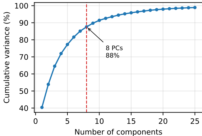
PCA on 62 log-SVI series
