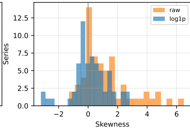
Effect of the log transform
