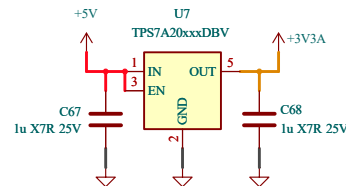
+3V3A LDO
