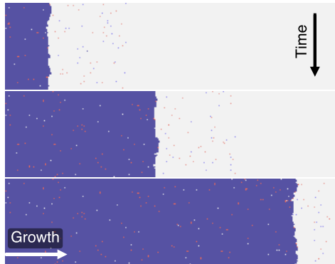
C High Supersaturation \beta\Delta\Phi , High Chemical Drive \beta\Delta\mu , Leading to Ordered and Fast Growth
