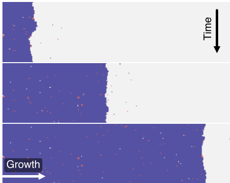
A Low Supersaturation \beta\Delta\Phi , No Chemical Drive \beta\Delta\mu , Leading to Ordered and Slow Growth
