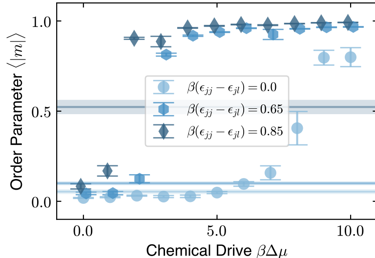
Heterogeneous Chemical Reactions \mathcal{S}5 \beta\Delta\Phi \approx 0.1
