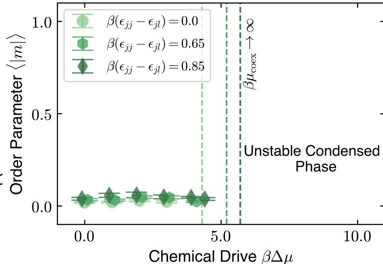
Homogeneous Chemical Reactions \mathcal{S}1 \beta\Delta\Phi \approx 0.1
