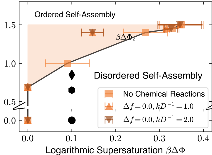
Numerical Phase Diagram for Reversible Chemical Reactions
