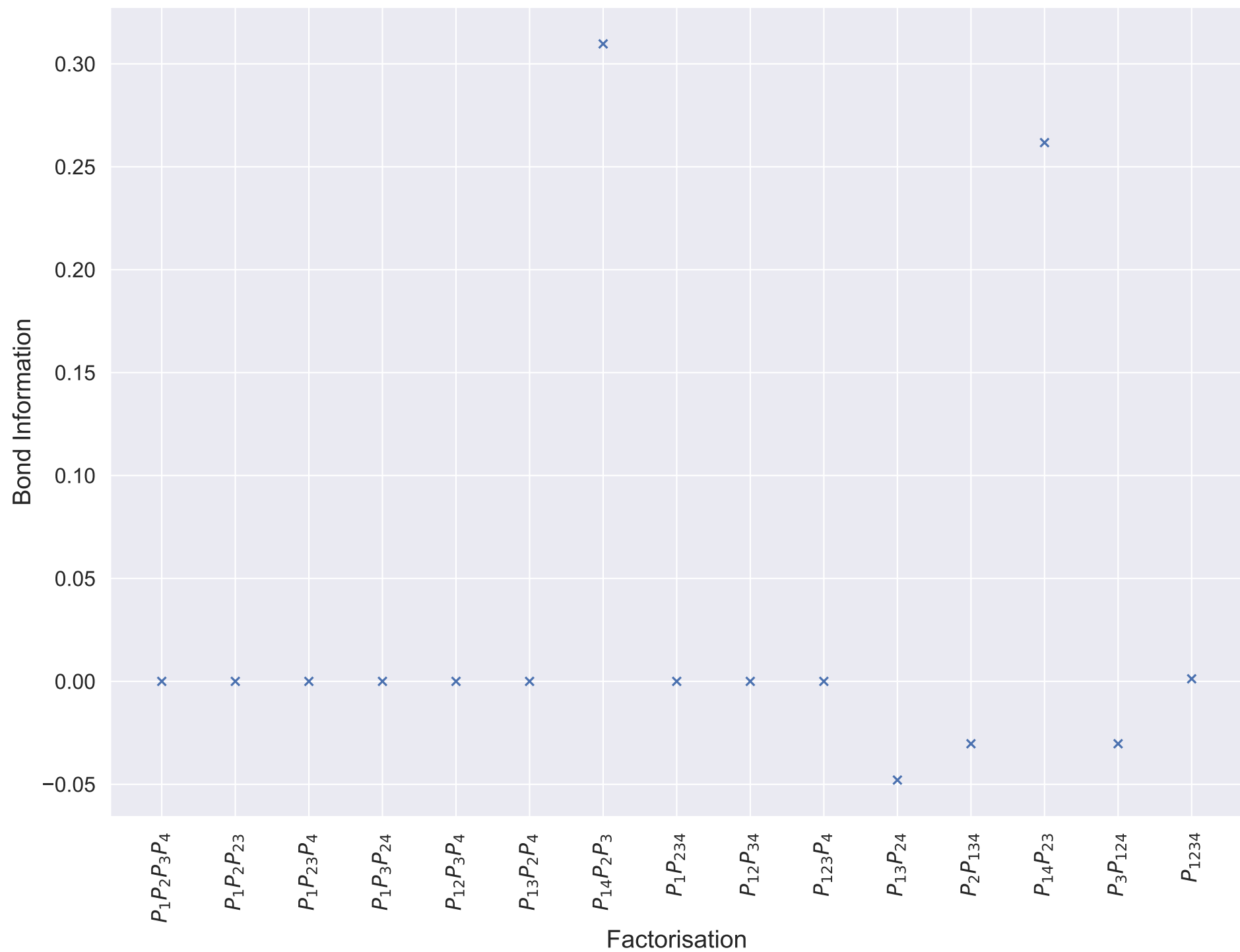
4-Variable Path Bond Information for Different Gaussian Factorisations
