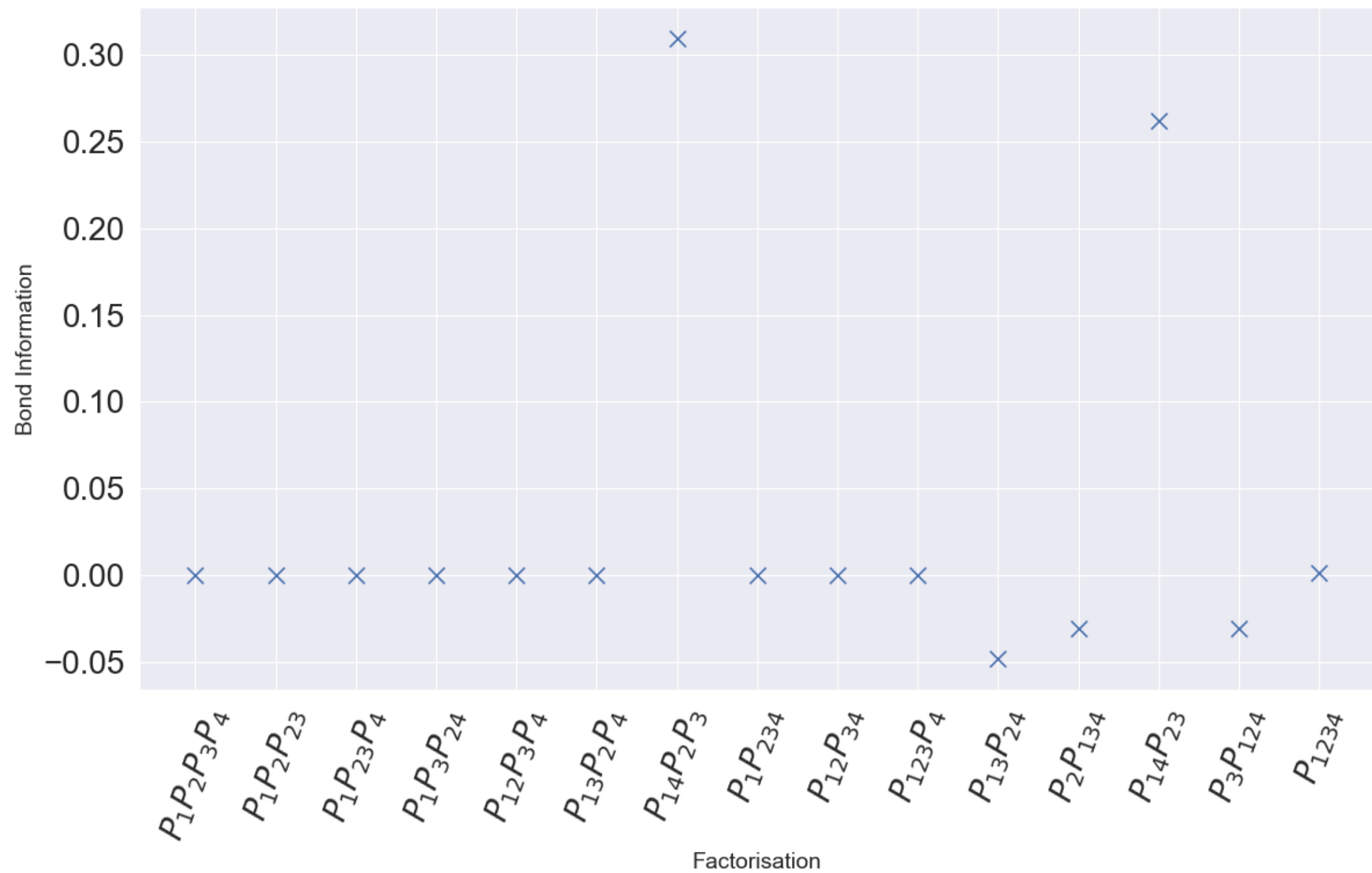
4-Variable Path Bond Information for Different Gaussian Factorisations
