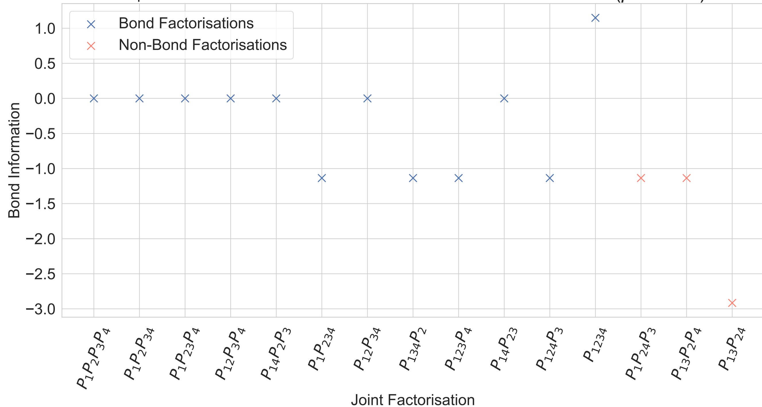
C_4 Bond Information for Different Gaussian Factorisations ( \rho = 0.99 )
