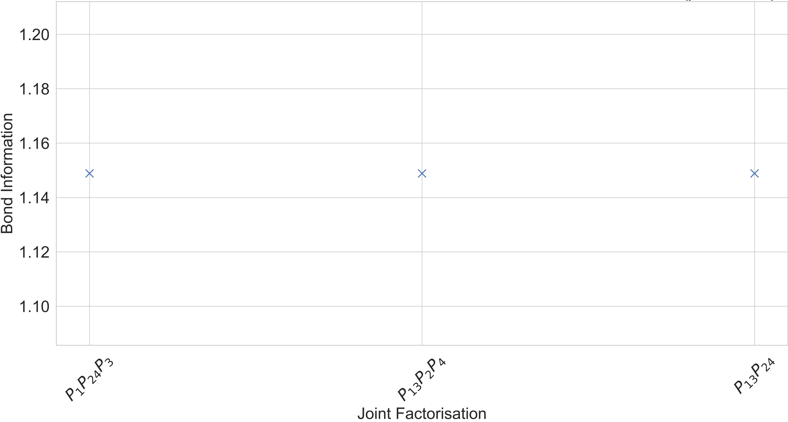
C_4 Bond Information for Non-Bond Factorisations of Joint Distribution ( \rho = 0.99 )
