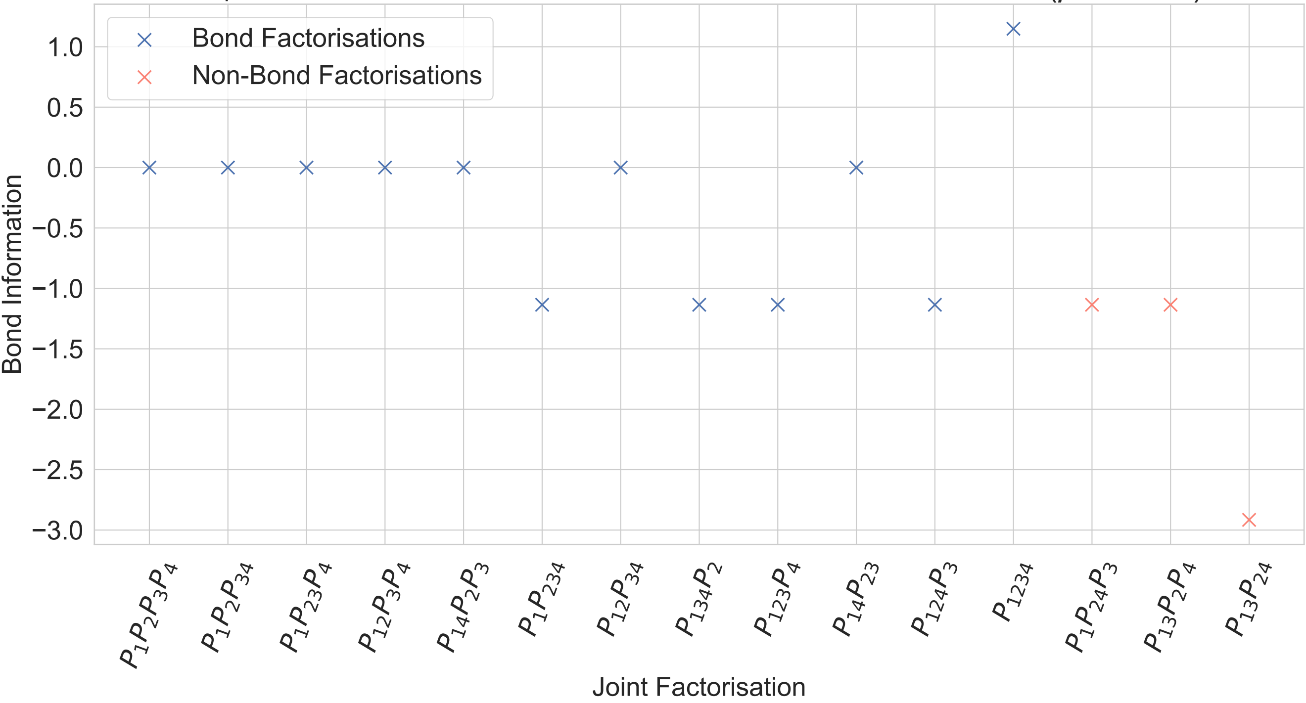
C_4 Bond Information for Different Gaussian Factorisations ( \rho = 0.99 )
