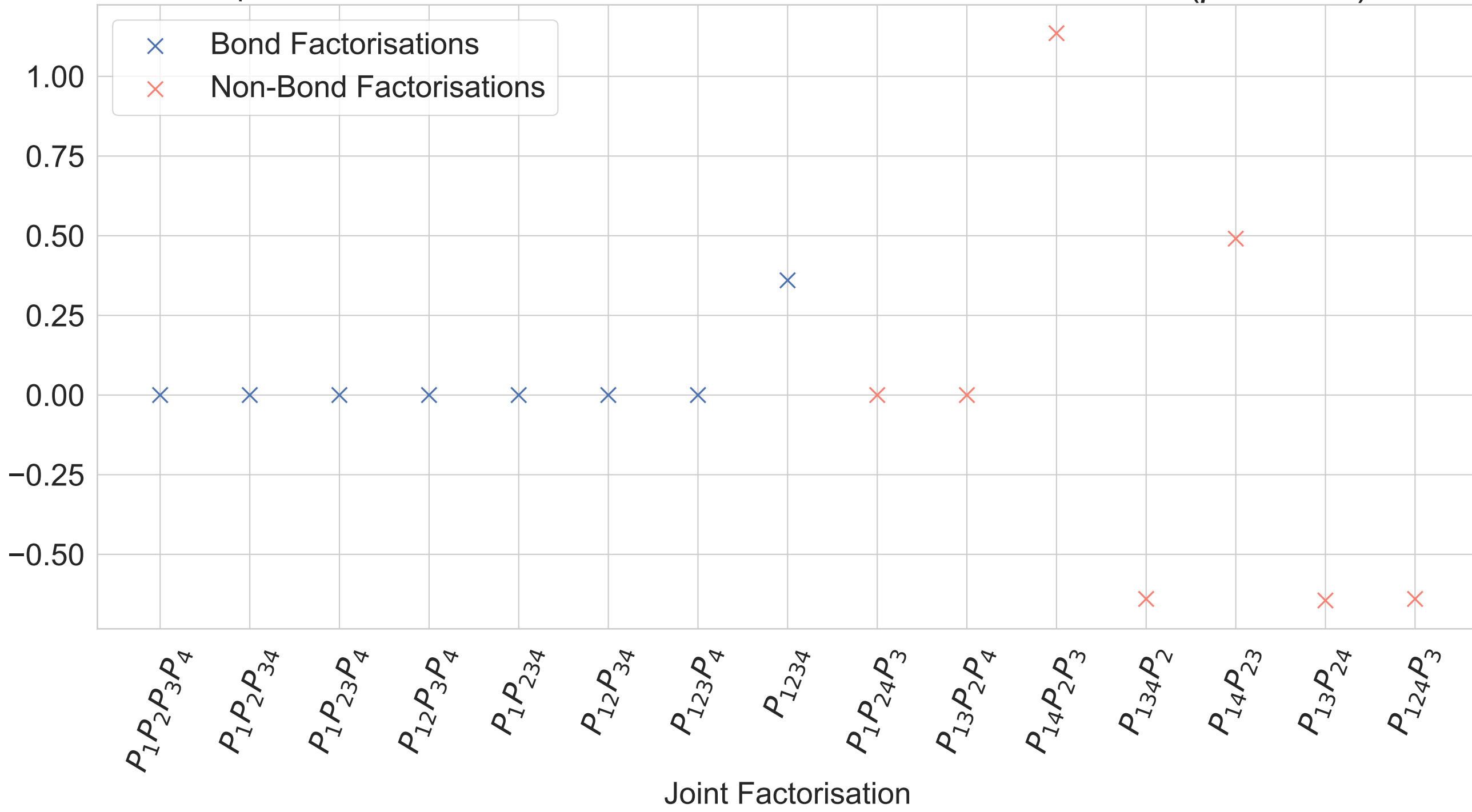
P_4 Bond Information for Different Gaussian Factorisations ( \rho = 0.99 )
