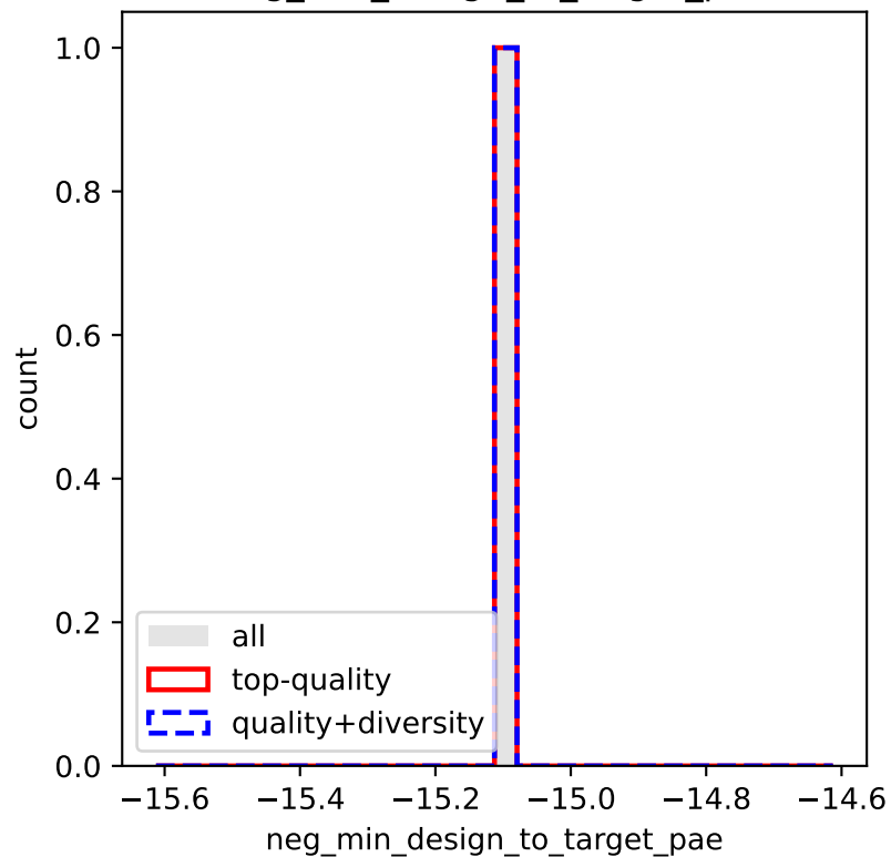
neg_min_design_to_target_pae
