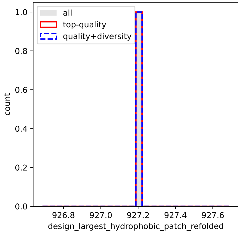
design_largest_hydrophobic_patch_refolded
