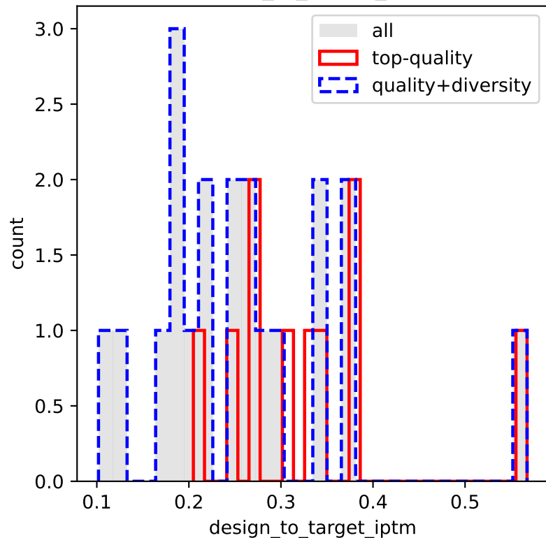
design_to_target_ipm
