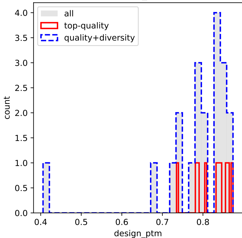
design_ptm
