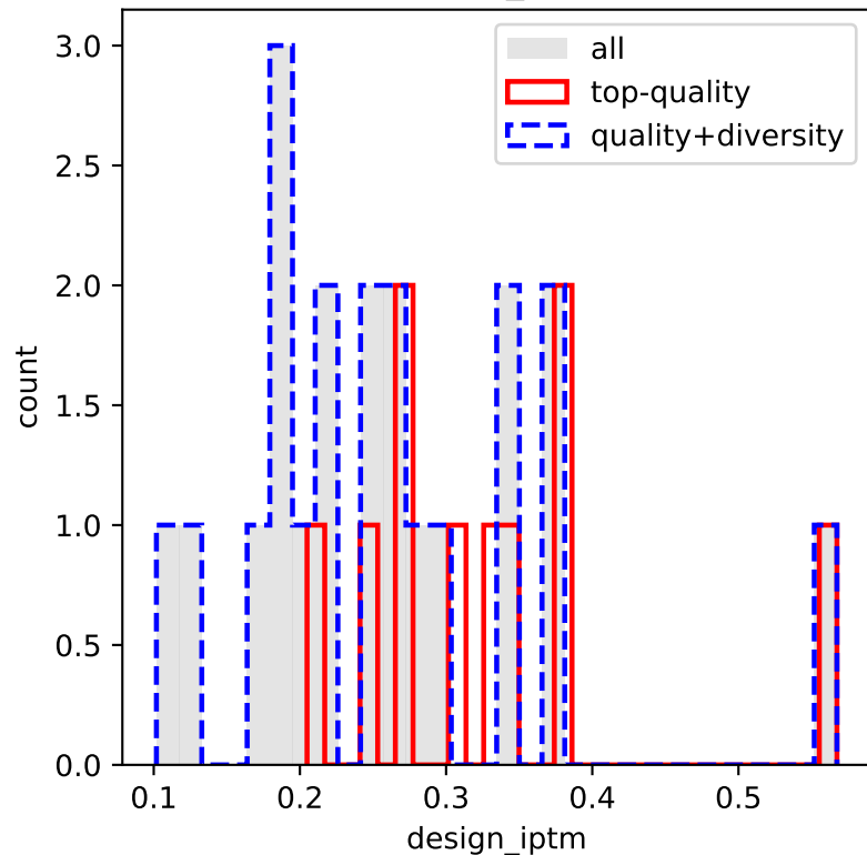
design_ipm
