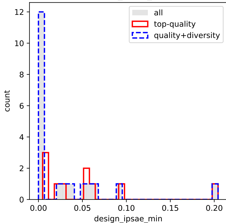
design_ipsae_min
