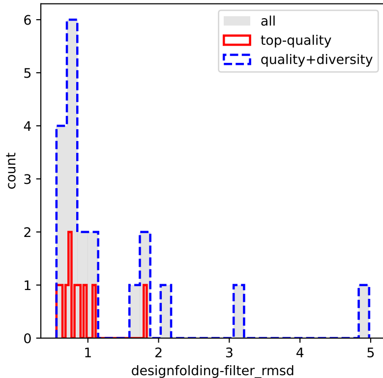
designfolding-filter_rmsd
