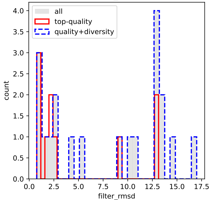
filter_rmsd
