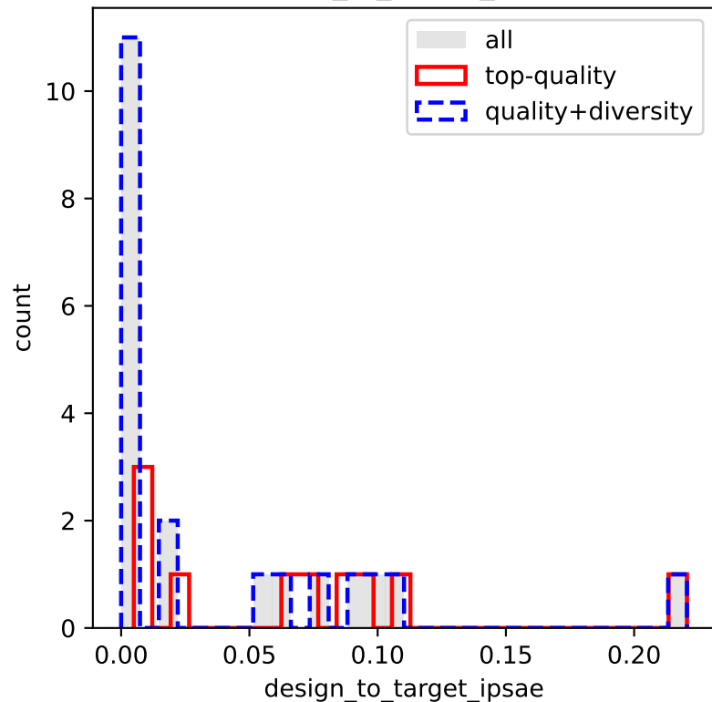
design_to_target_ipsae
