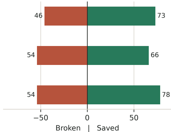
Exact Mutation
