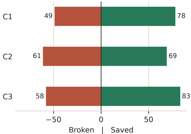
DB Match
