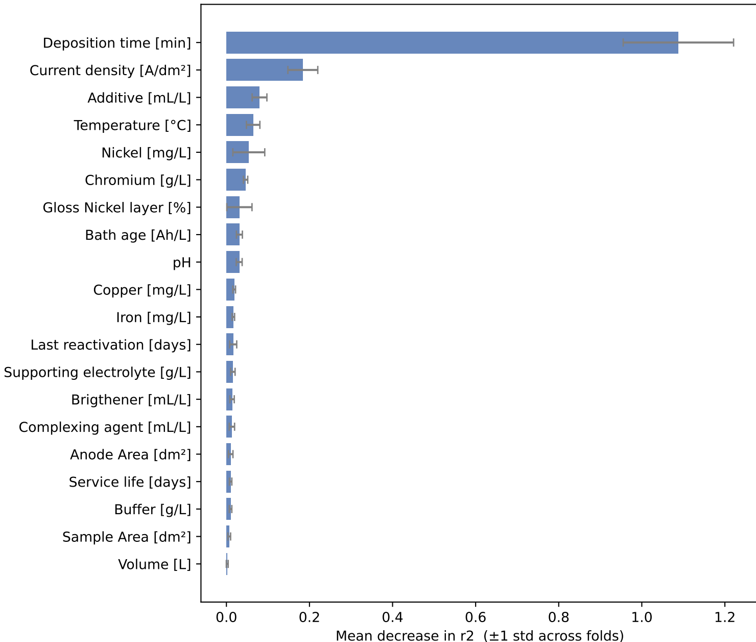
CV Permutation Importance [5 folds] Regression
