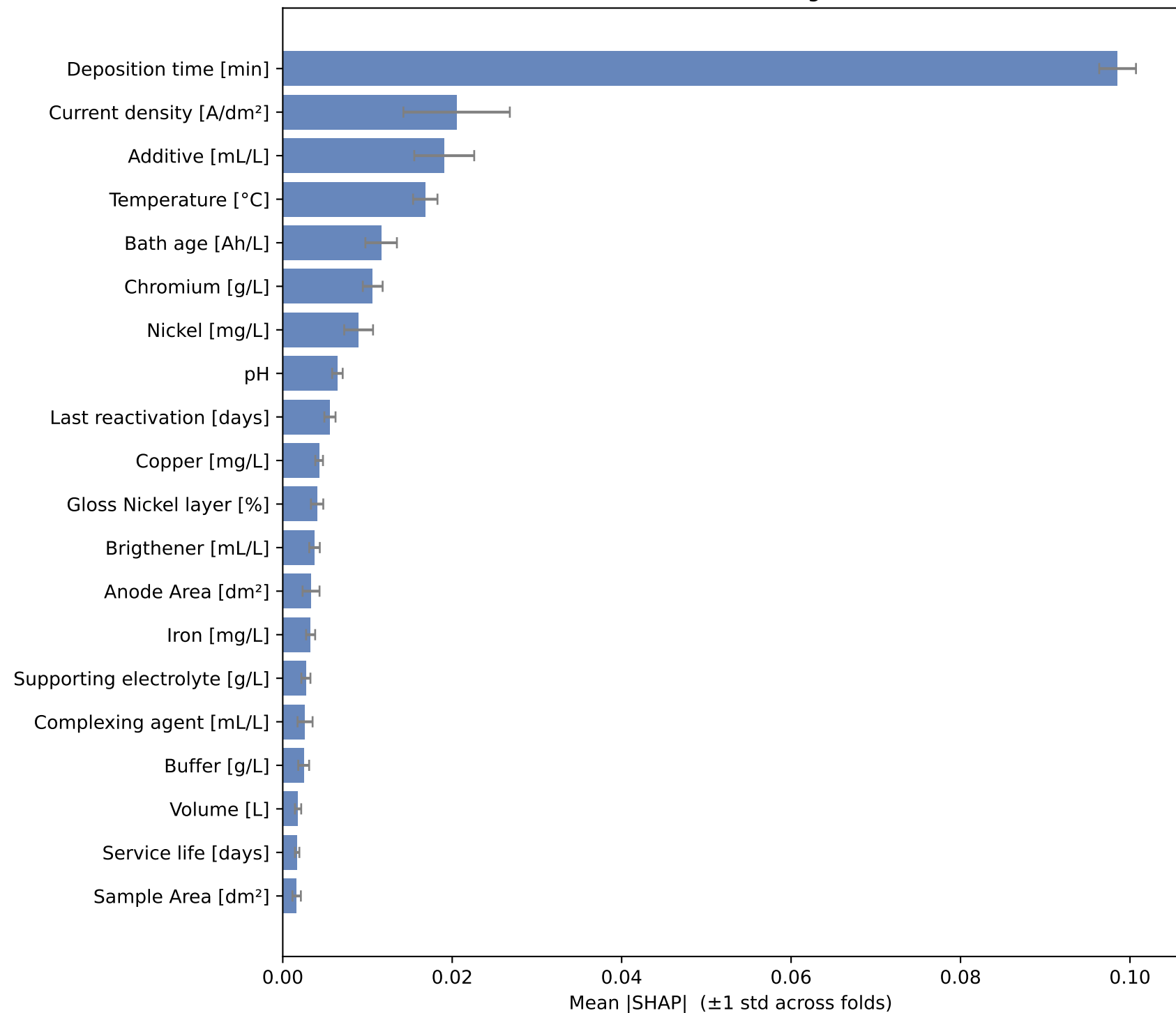
CV SHAP [5 folds] Regression
