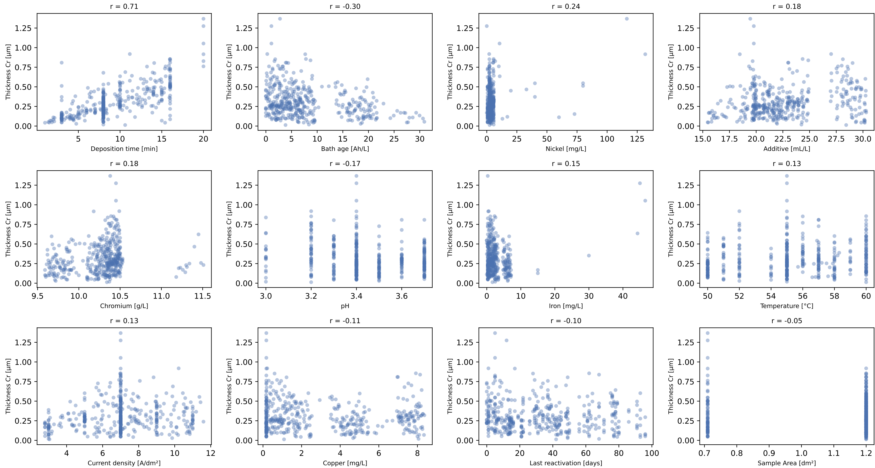
Target vs. Top 12 Features (by |r|)
