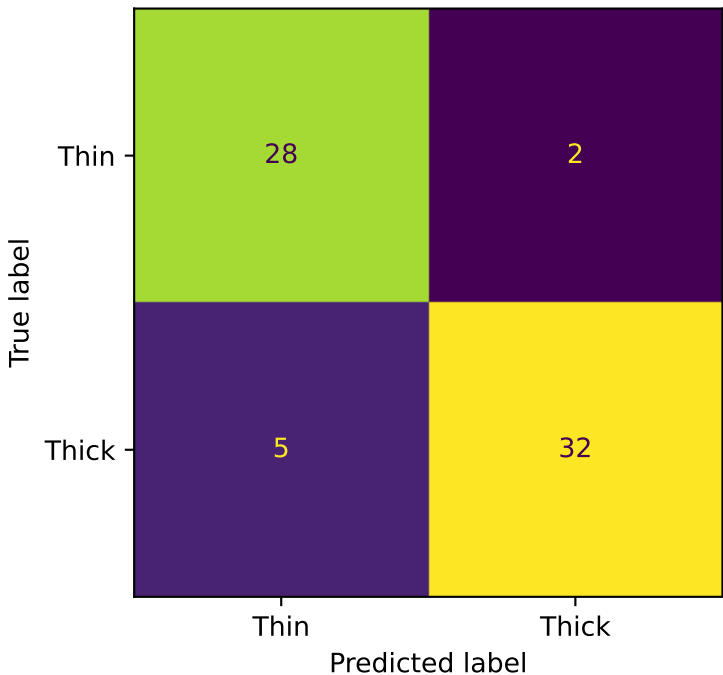
Confusion Matrix — ensemble:averaging
