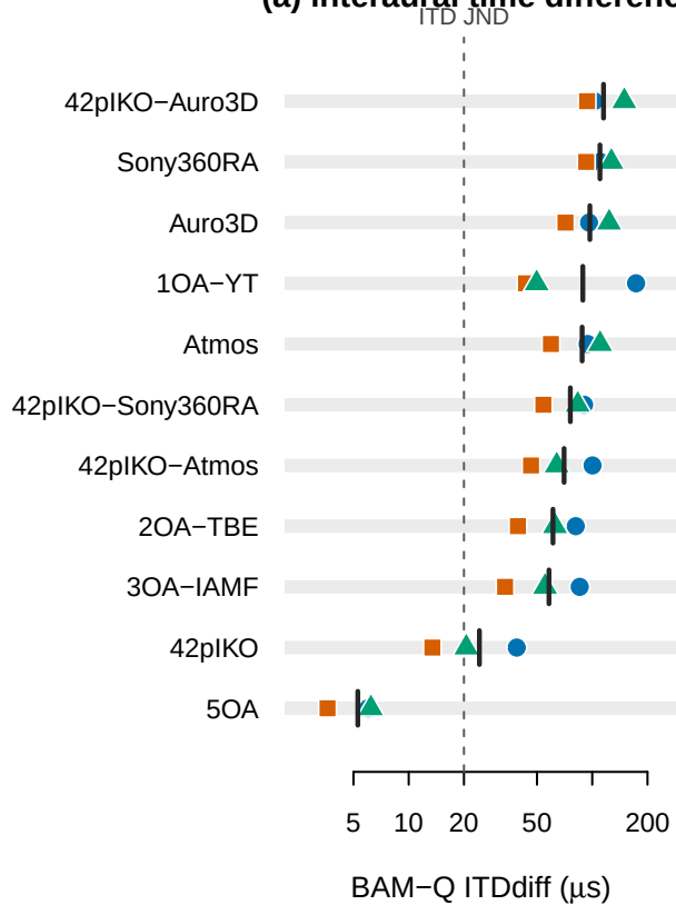
(a) interaural time difference
