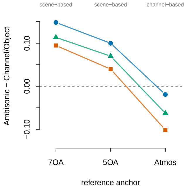
(b) BINAQUAL LS
