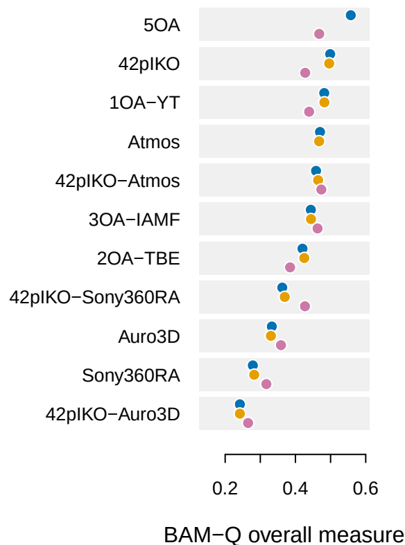
(a) perceptual quality
