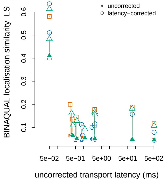
(a) BINAQUAL
