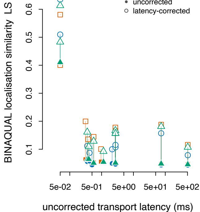
(a) BINAQUAL
