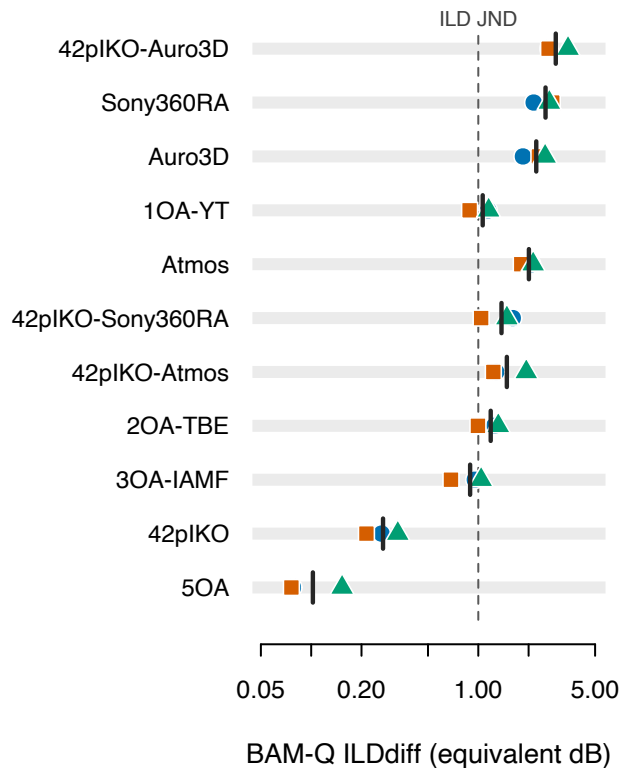
(b) interaural level difference
