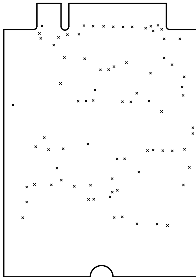
Drill Map: × 0,300mm / 0,0118" (80 holes)
