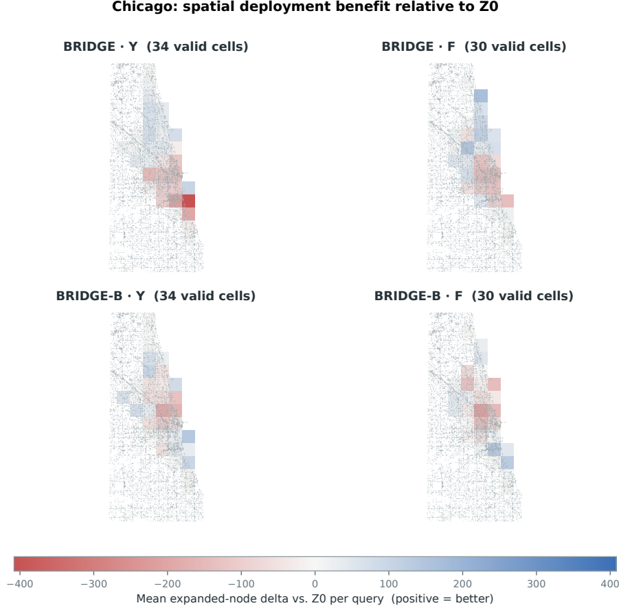
Figure C.7: Chicago: per-query expanded-node differences of BRIDGE and BRIDGE-B against Z0 in Y/F . Positive and negative cells coexist — local improvements do not add up to a city-wide advantage.
