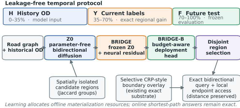
Figure 1: End-to-end pipeline. The overlay substrate is an existing exact index structure; this paper studies historical-OD-driven region ranking, isolation, and selective materialization. Learning allocates offline resources only — online queries stay exact.
