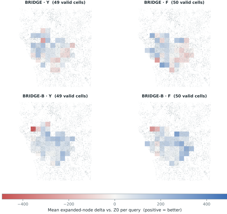
Figure C.6: Porto: per-query expanded-node differences of BRIDGE and BRIDGE-B against Z0 in Y/F , on the spatial grid. Blue means the neural method expands fewer nodes; BRIDGE-B's positive coverage is broad in both windows.
