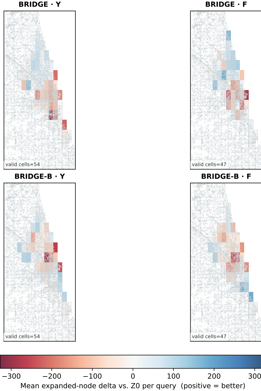
Figure C.7: Chicago: per-query expanded-node differences of BRIDGE and BRIDGE-B against Z0 in Y/F. Positive and negative cells coexist — local improvements do not add up to a city-wide advantage.
