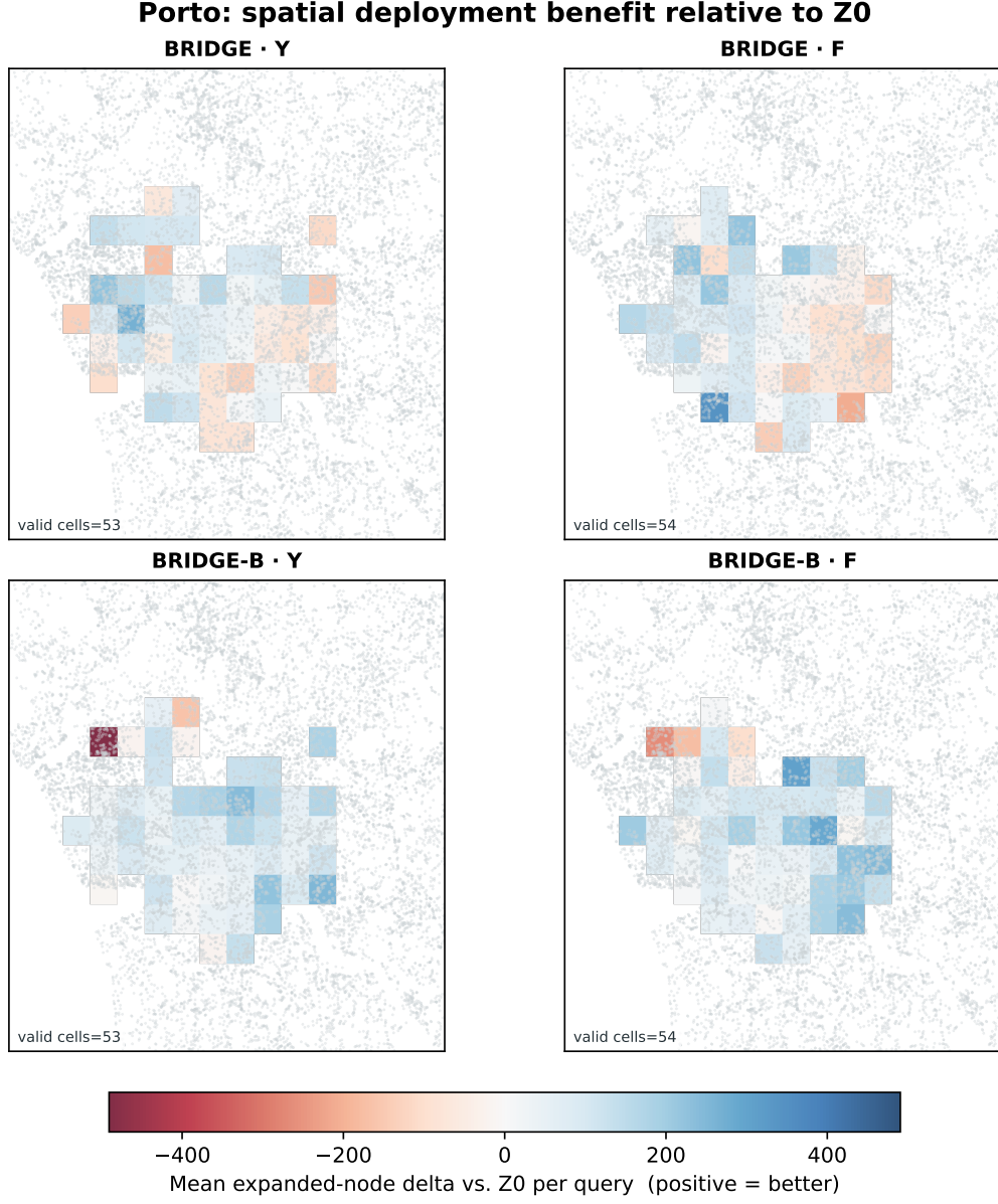
Figure C.6: Porto: per-query expanded-node differences of BRIDGE and BRIDGE-B against Z0 in Y/F , on the spatial grid. Blue means the neural method expands fewer nodes; BRIDGE-B's positive coverage is broad in both windows.
