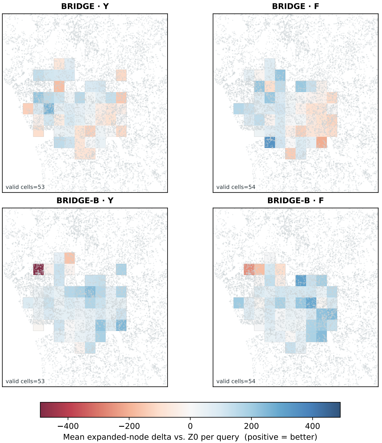
Figure C.6: Porto: per-query expanded-node differences of BRIDGE and BRIDGE-B against Z0 in Y/F , on the spatial grid. Blue means the neural method expands fewer nodes; BRIDGE-B's positive coverage is broad in both windows.
