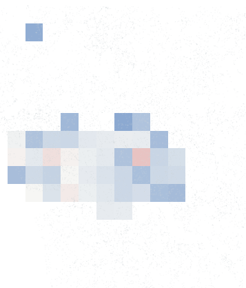
BRIDGE-B · Y-O 44 valid cells
