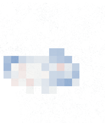
BRIDGE-B · F-O 43 valid cells
