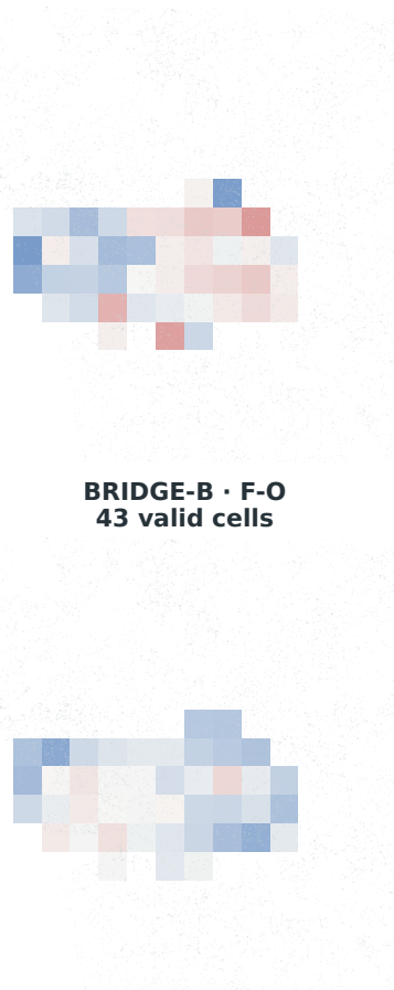
BRIDGE · F-O 43 valid cells
