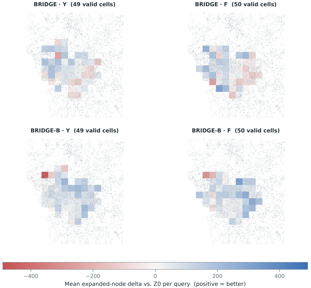
Figure C.6: Porto: per-query expanded-node differences of BRIDGE and BRIDGE-B against Z0 in Y/F , on the spatial grid. Blue means the neural method expands fewer nodes; BRIDGE-B's positive coverage is broad in both windows.
