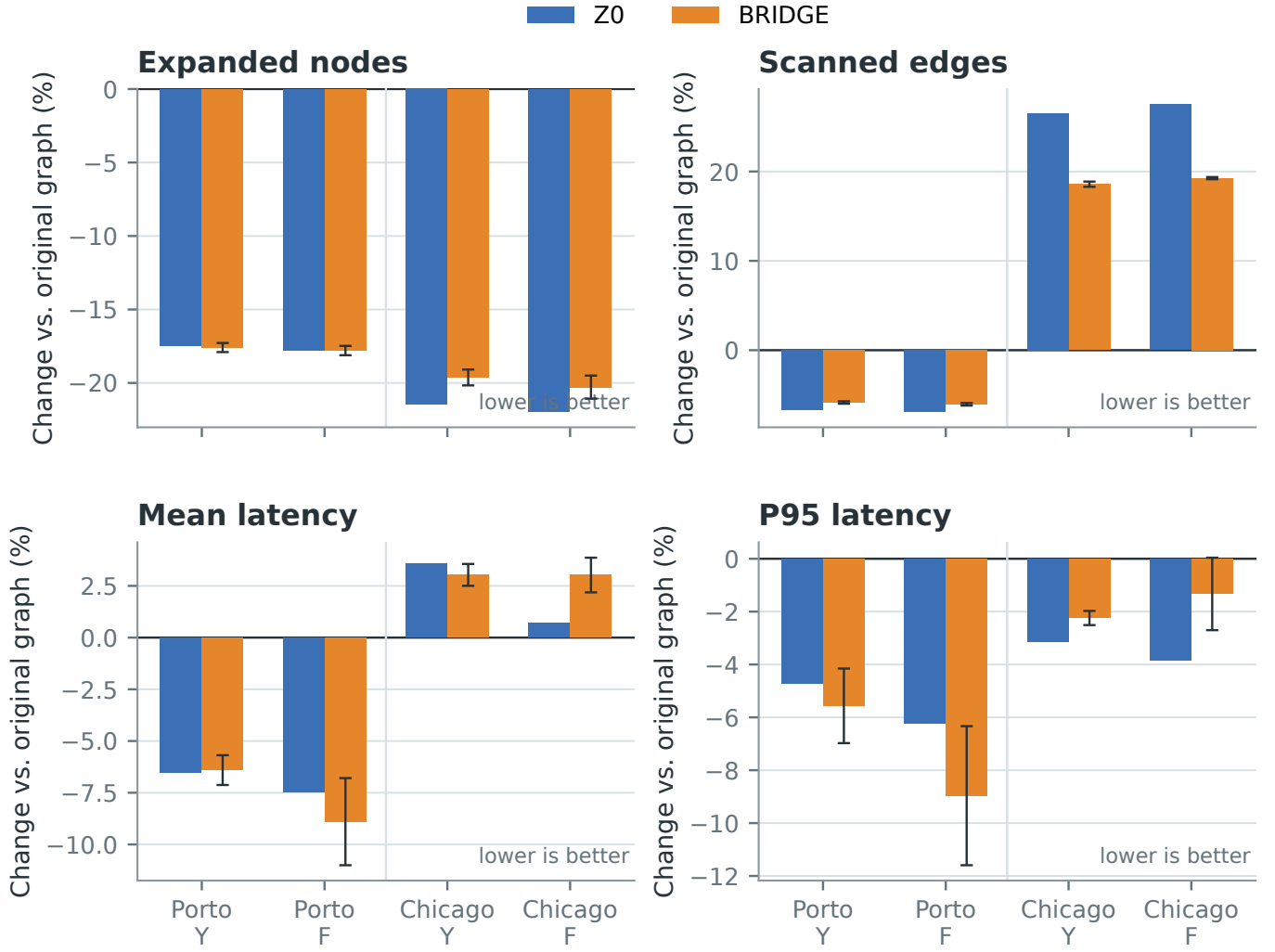
Figure 4: System gains and costs of selective materialization in both cities under one C++20/O3 implementation. Negative means a reduction relative to the original graph. Chicago expands fewer nodes yet scans more edges through dense shortcuts — ranking gains and wall-clock gains are not the same thing.
