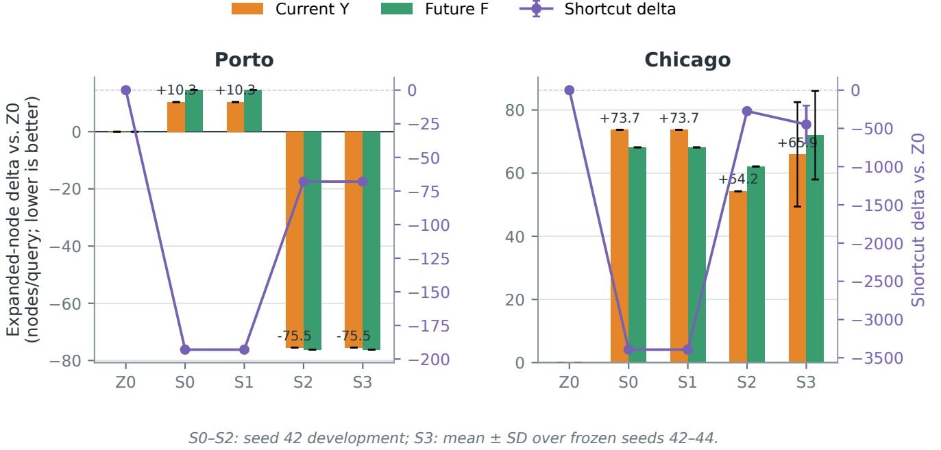
Figure 5: BRIDGE-B’s real deployment trajectory from S0 to S3. S0-S2 are seed-42 development stages; S3 shows the frozen protocol over seeds 42/43/44 with means and population standard deviations. Porto improves with zero variance; Chicago stably cuts shortcuts and holds the head; both cities stay within 3% of Z0 in online expansions.
