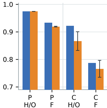
NDCG@18
