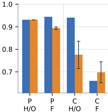
NDCG@5
