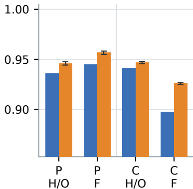
Spearman
