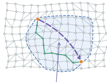
(c) Materialized shortcut
