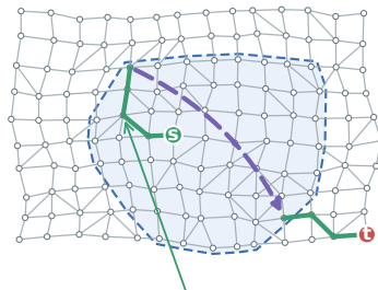
(e) One endpoint inside
