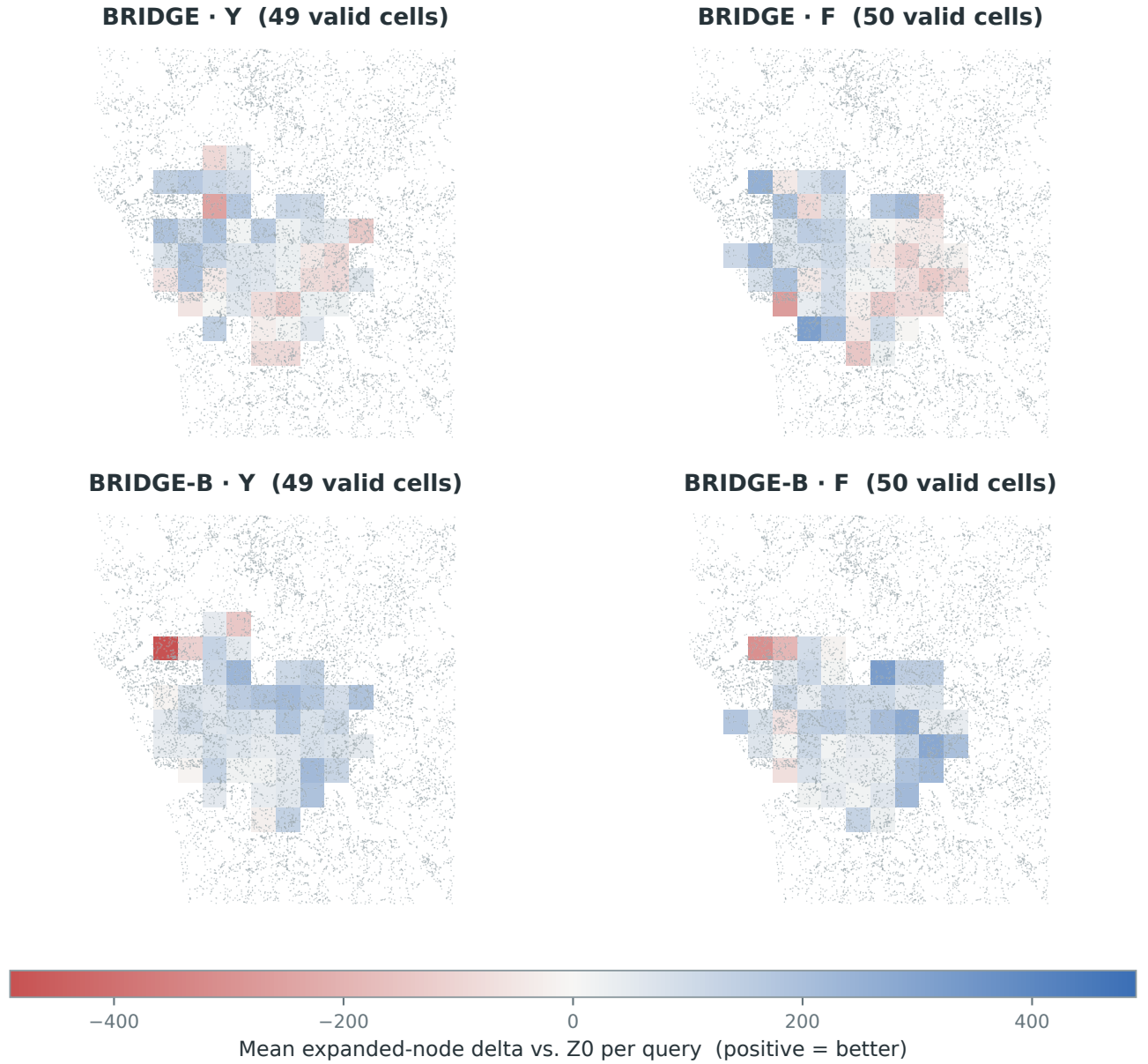
Figure C.7: Porto: per-query expanded-node differences of BRIDGE and BRIDGE-B against Z0 in Y/F , on the spatial grid. Blue means the neural method expands fewer nodes; BRIDGE-B's positive coverage is broad in both windows.
