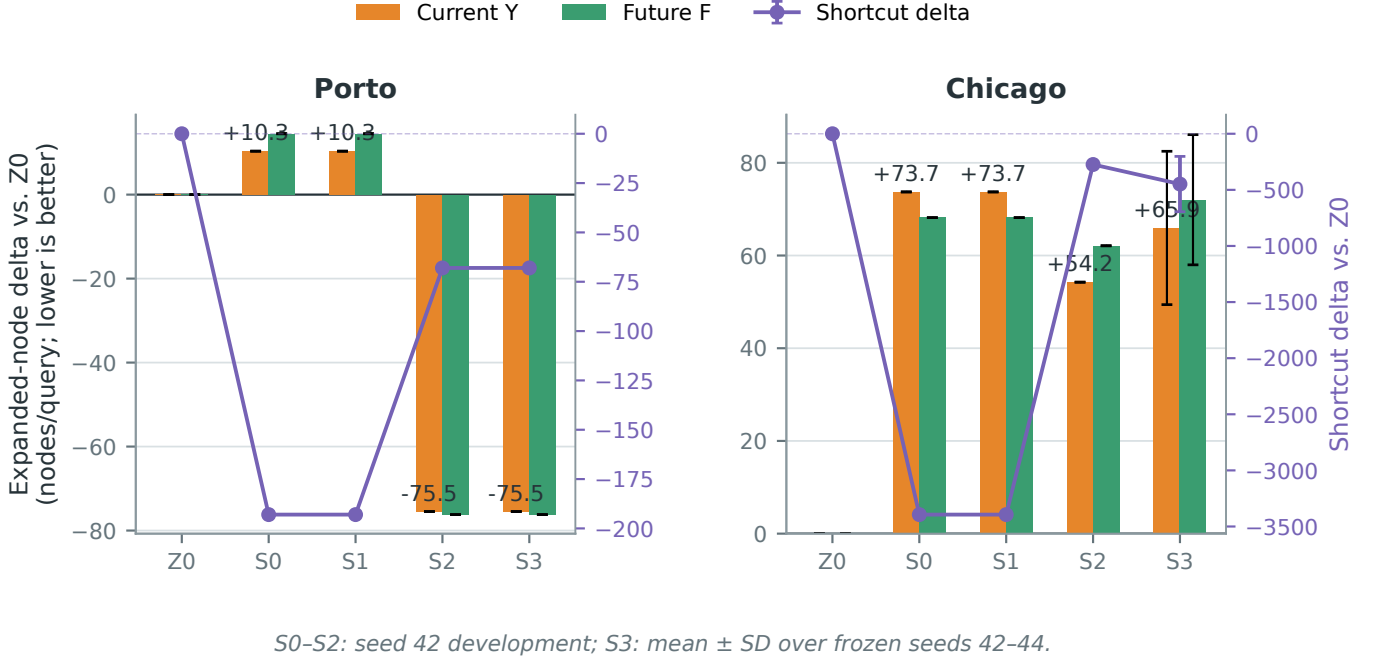
Figure 6: BRIDGE-B’s real deployment trajectory from S0 to S3. S0-S2 are seed-42 development stages; S3 shows the frozen protocol over seeds 42/43/44 with means and population standard deviations. Porto improves with zero variance; Chicago stably cuts shortcuts and holds the head; both cities stay within 3% of Z0 in online expansions.
