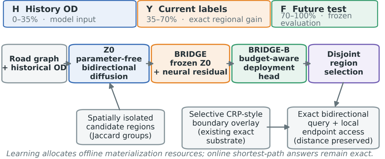
Figure 2: End-to-end pipeline. The overlay substrate is an existing exact index structure; this paper studies historical-OD-driven region ranking, isolation, and selective materialization. Learning allocates offline resources only — online queries stay exact.
