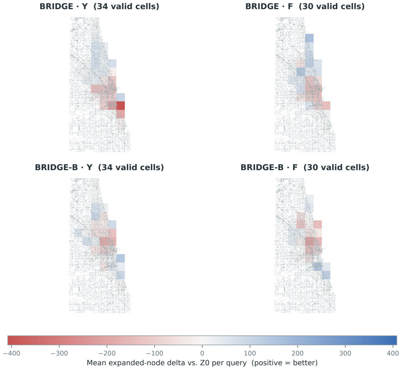
Figure C.8: Chicago: per-query expanded-node differences of BRIDGE and BRIDGE-B against Z0 in Y/F . Positive and negative cells coexist — local improvements do not add up to a city-wide advantage.
