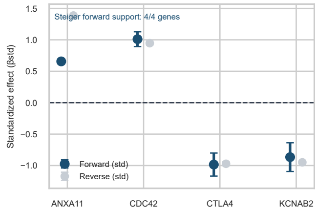
Panel D Directionality supports gene \rightarrow phenotype
