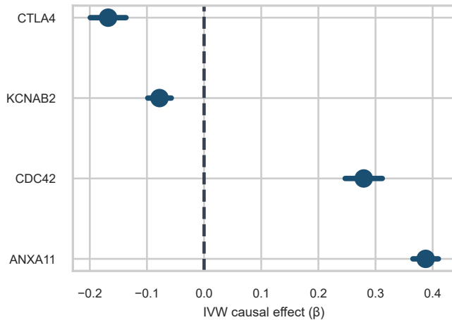
Panel C Leave-one-out robustness
