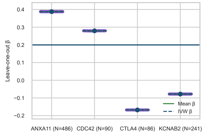
Panel C Leave-one-out robustness
