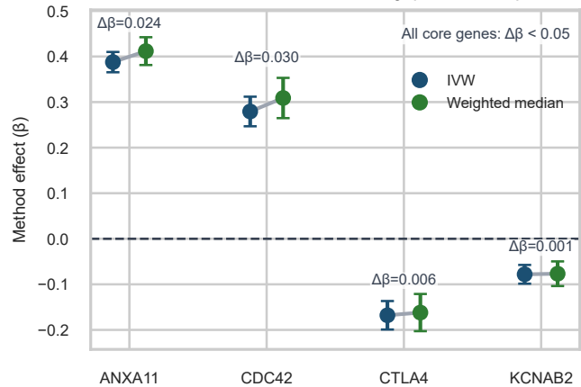
Panel B Method consistency (IVW vs WM)
