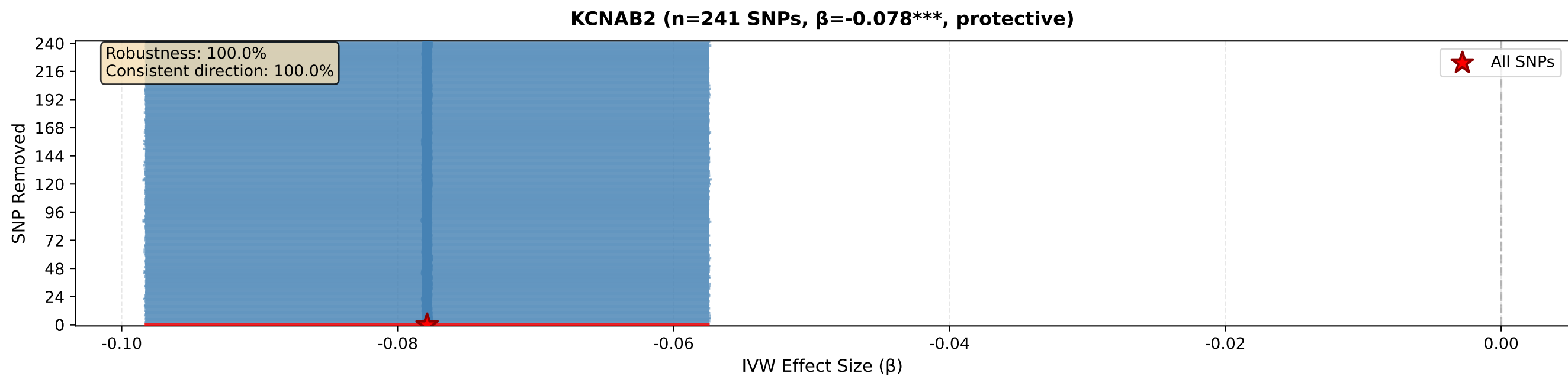
Figure S10: Leave-one-out Sensitivity Analysis
