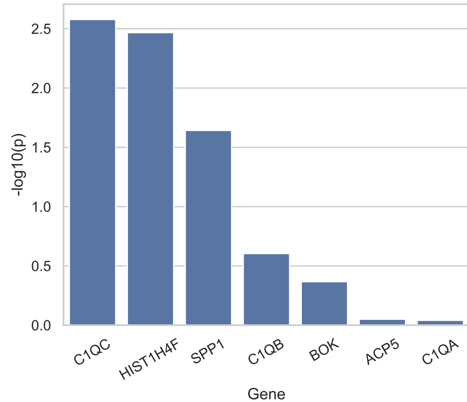
Specificity ranking
