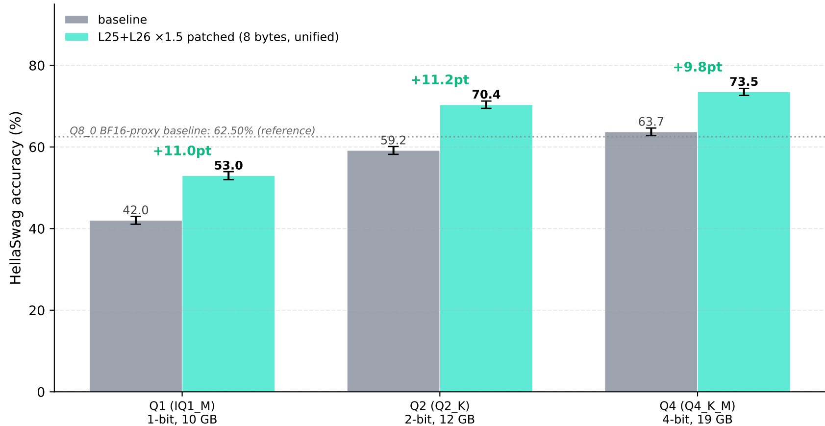
Gemma 4 31B: 8-byte L25+L26 patch HellaSwag improvement (3 release quants, n=10,042 full, Wilson 95% CI; Q8 baseline = reference line)
