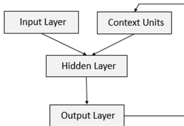
Figure 1 – Jordan recurrent neural network
