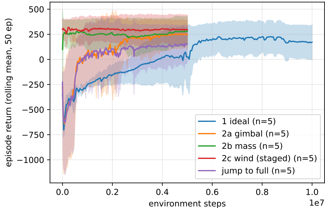
Training return
