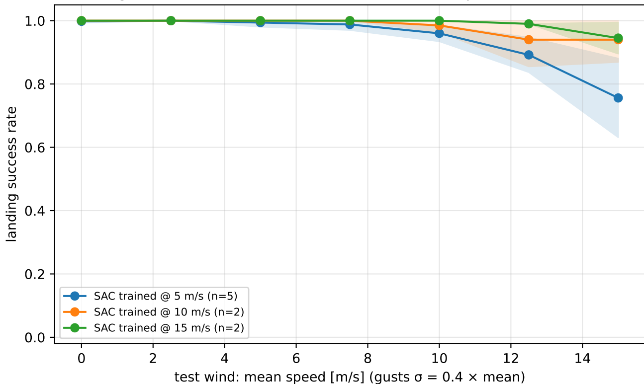
SAC generalisation to unseen wind levels (100 episodes/seed/level)
