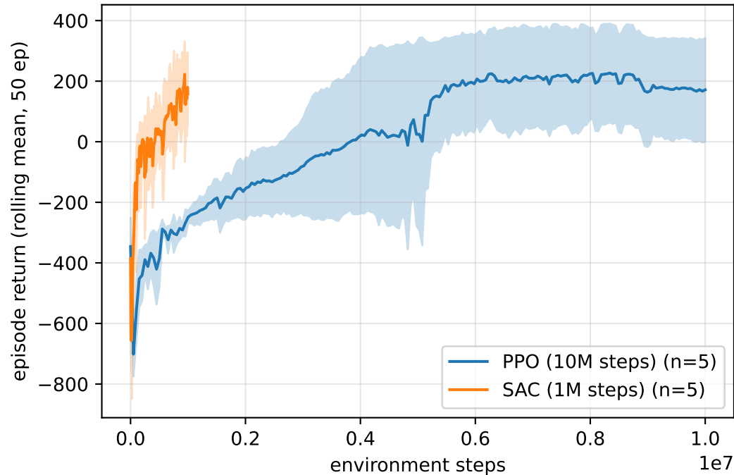
Training return
