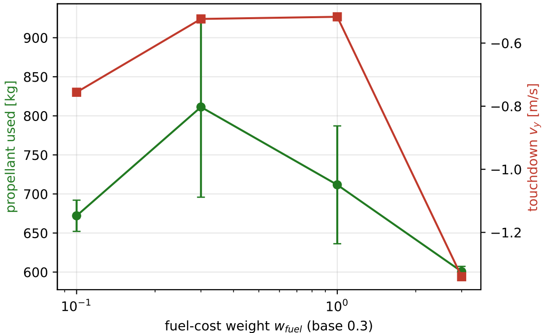
SAC fuel-economy vs touchdown-softness trade-off
