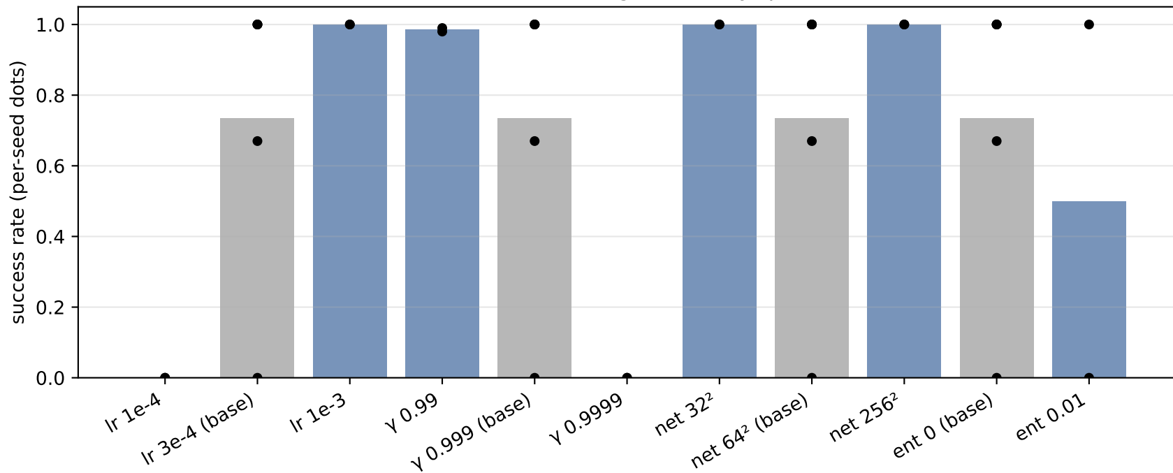
PPO from-scratch learning sensitivity (phase-1 env)
