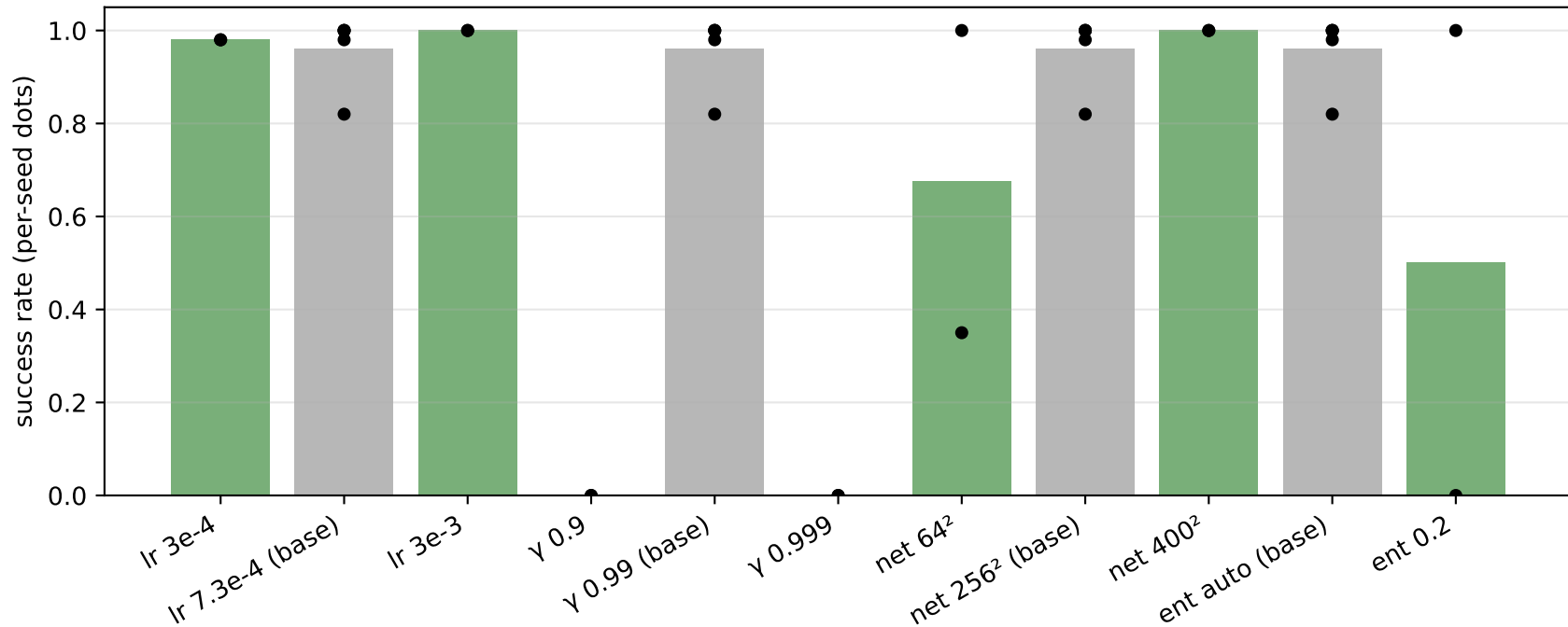
SAC from-scratch learning sensitivity (phase-1 env)
