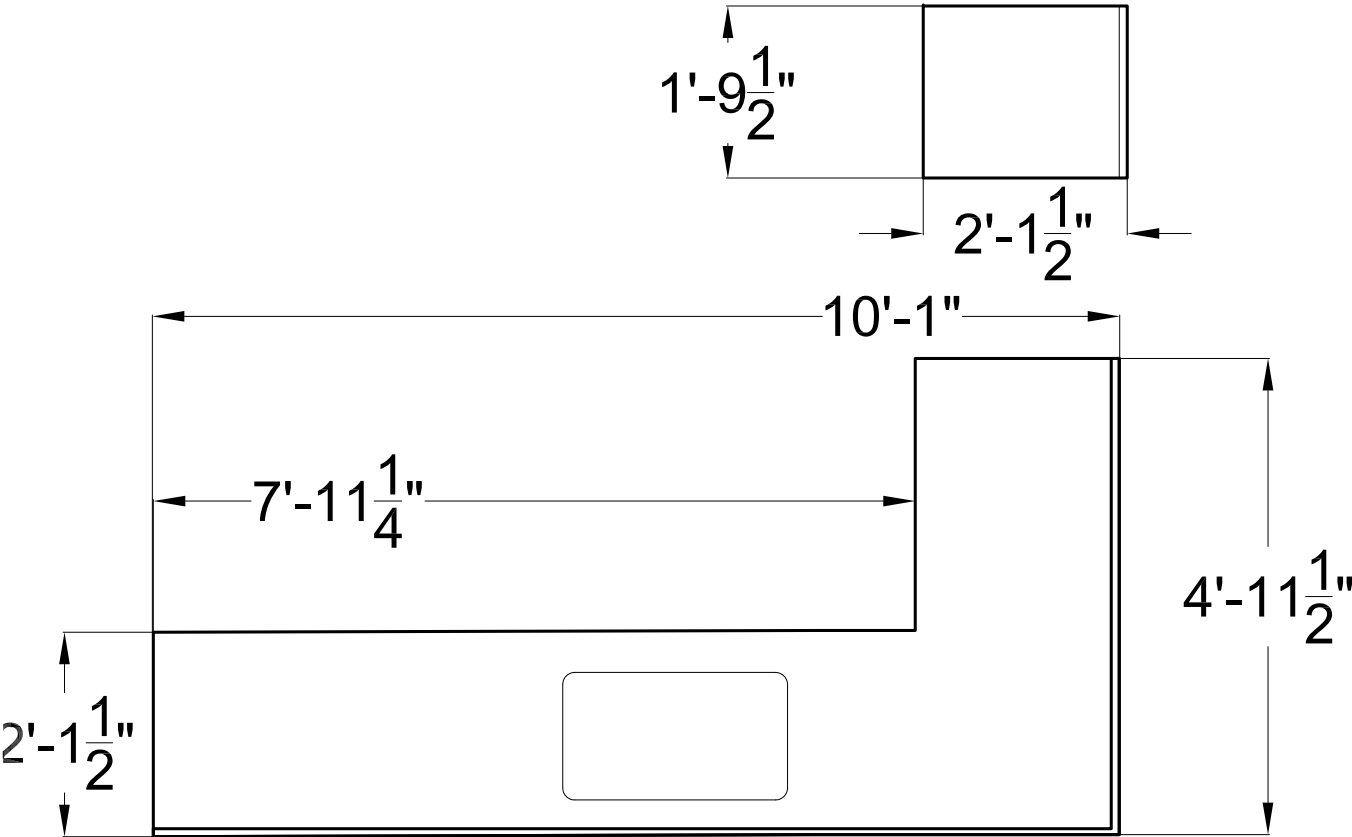
UNIT 2 COUNTERTOP PLAN
