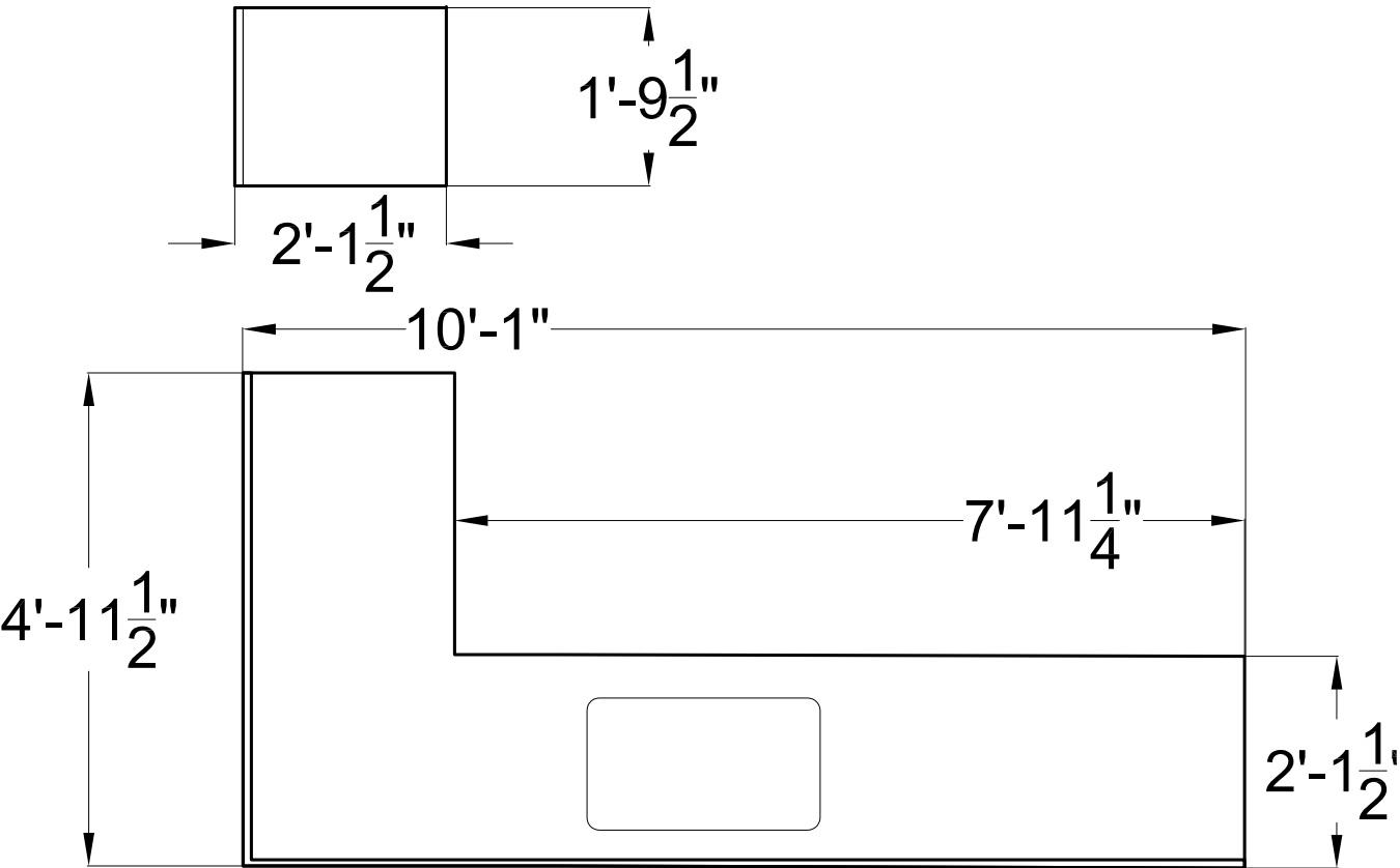
UNIT 1 COUNTERTOP PLAN
