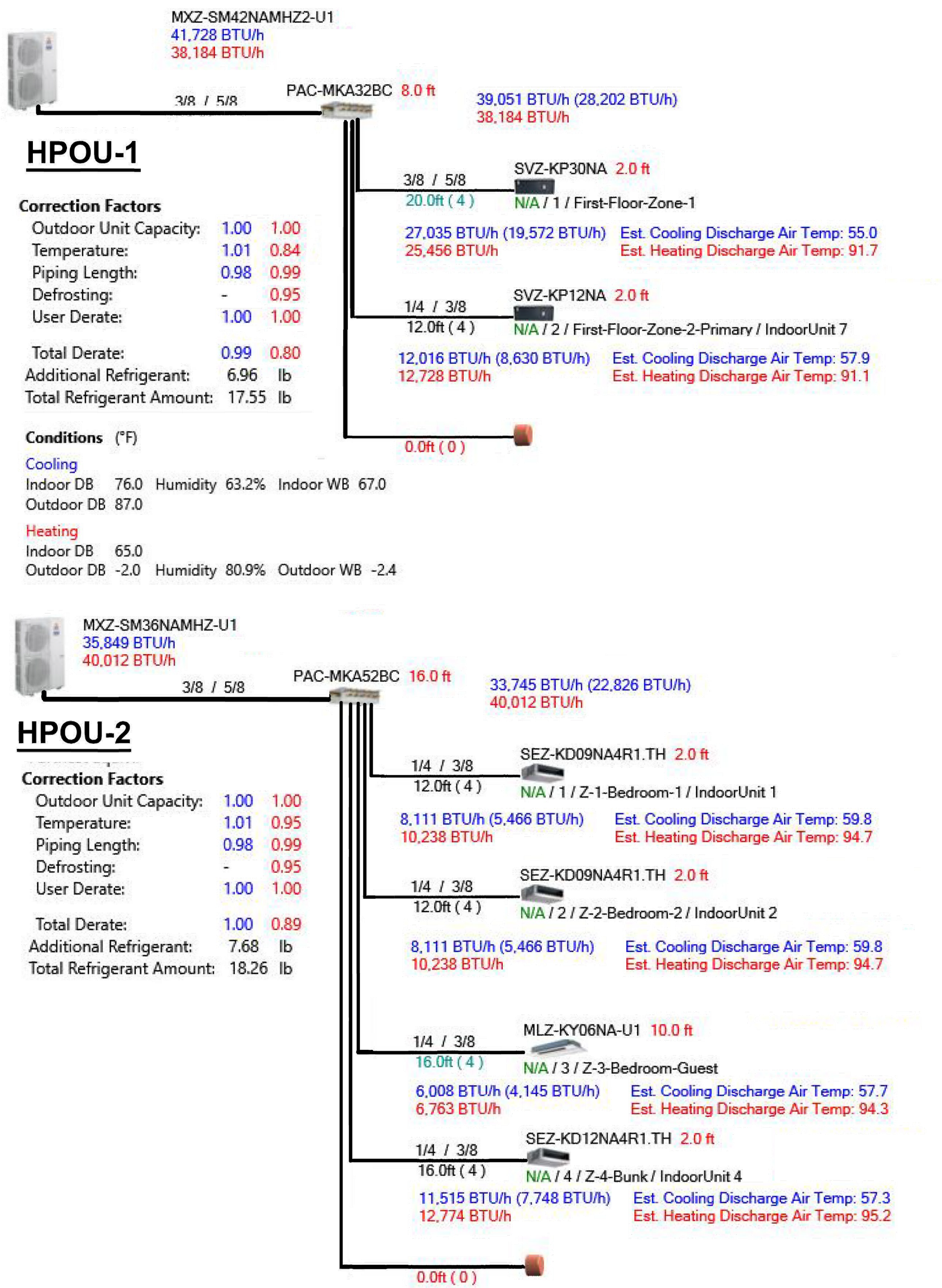
HEAT PUMP SYSTEM SCHEMATICS SCALE: NONE
