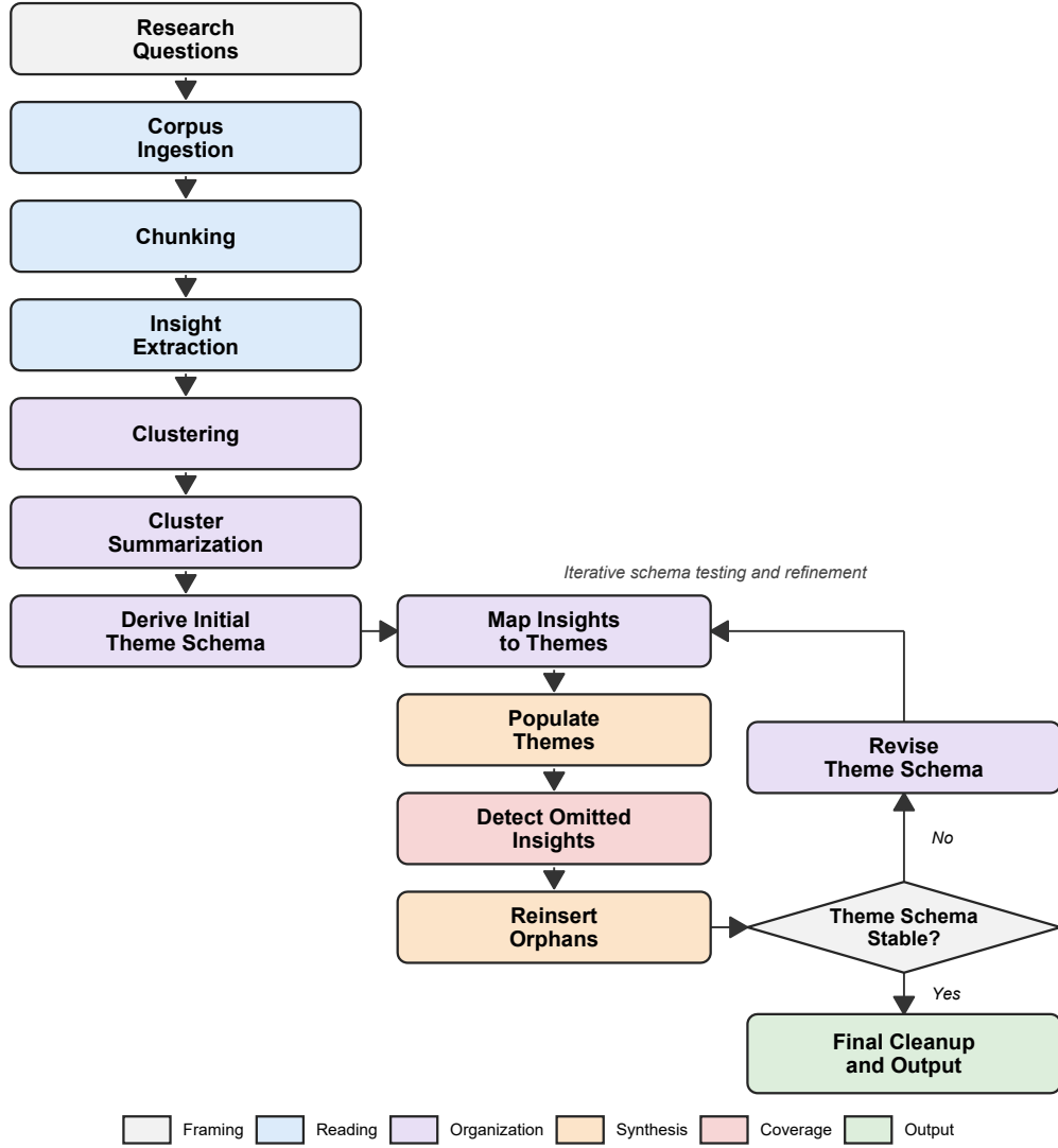
Figure 1: The system decomposes corpus analysis into structured reading stages, extracting atomic insights prior to synthesis. Clustering provides semantic scaffolding for theme generation, while synthesis occurs at the theme level. An explicit orphan detection and reinsertion mechanism enforces coverage, and an iterative loop refines the thematic schema until stable.
